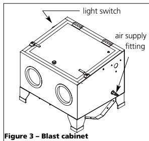
Figure 3 - Blast cabinet
