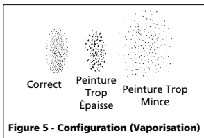
Figure 5 - Configuration (Vaporisation)
