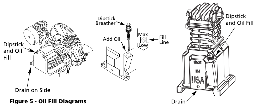
Figure 5 - Oil Fill Diagrams
