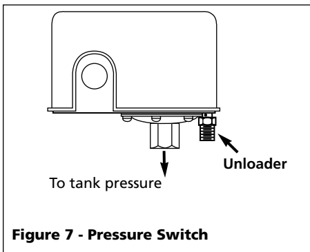
Figure 7 - Pressure Switch
