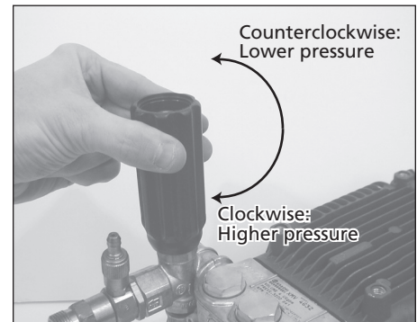
Figure 8 - Camshaft pump pressure adjustment
