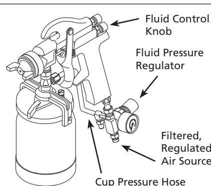
Figure 3 - Pressure Feed Cup Set-up
