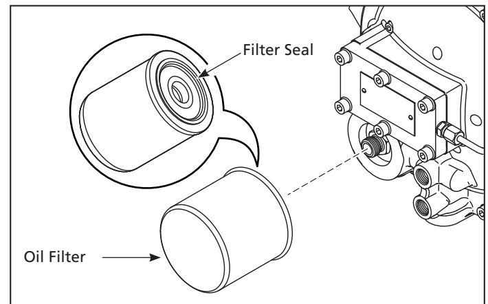
Figure 12 - Oil Filter
