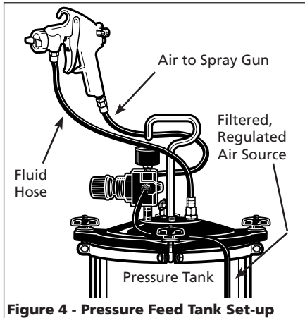
Figure 4 - Pressure Feed Tank Set-up
