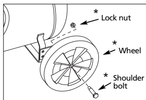
Figure 2 - Wheel Assembly
