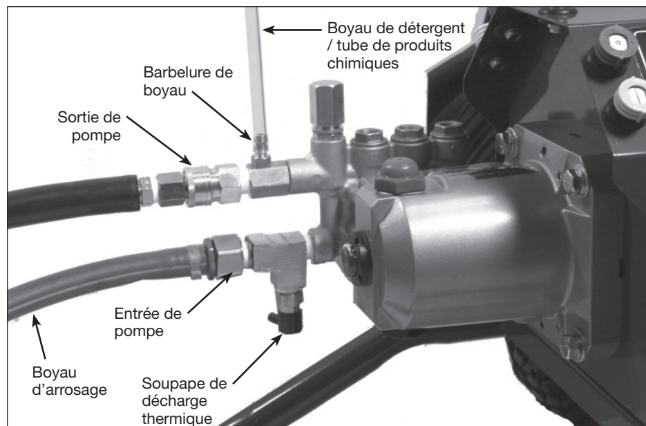
Figure 12 - Raccord de pompe
