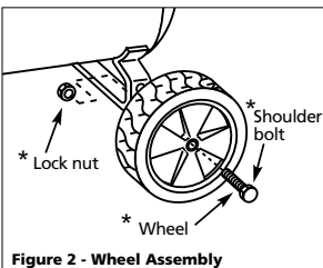
Figure 2 - Wheel Assembly
