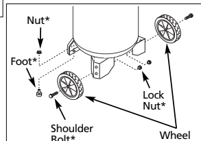
Figure 2 - Foot and Wheel Assembly
